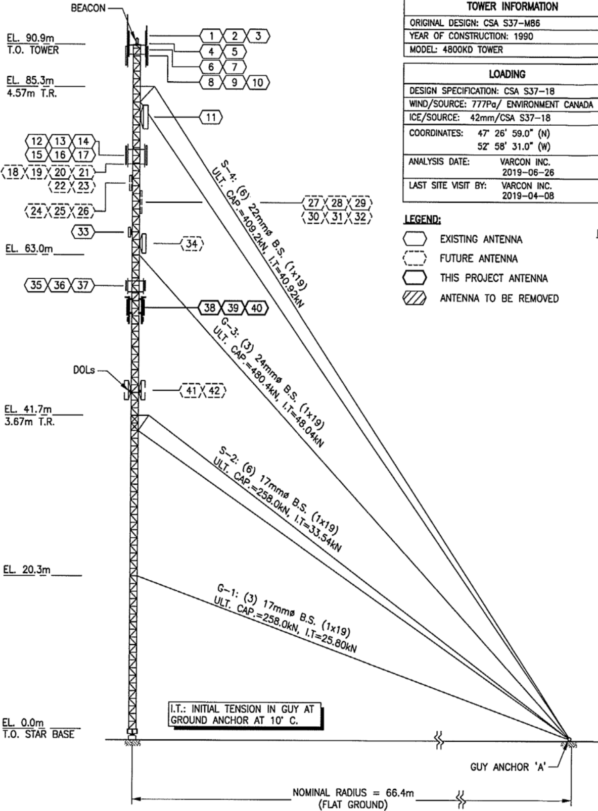
TOWER PROFILE SCALE 1:450 (11"x17" SHEET)
